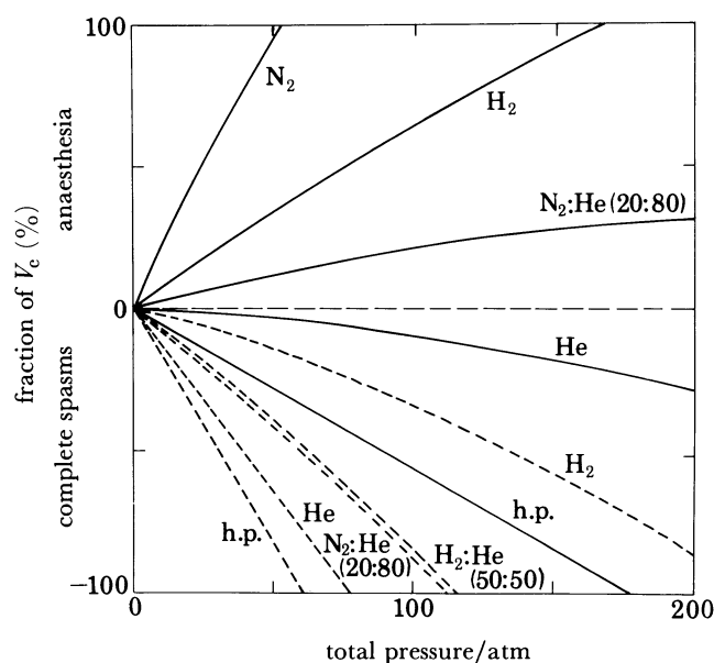
FIGURE 7. The ability of some gases and their mixtures to cause either general anaesthesia (solid lines) or complete spasms (broken lines) has been calculated from (1) and (2) with the corrections described previously (Miller et al. 1973; Miller 1977). The expansion (1) has been normalized to a percentage of the respective critical volumes. Parameters for the calculations have been given (Miller et al. 1978). Abbreviation: h.p., high pressure.
