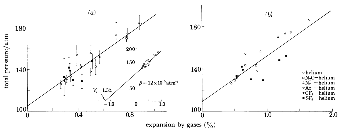
FIGURE 4. The data for non-tonic death from figure 2( d ) are used to test the predictions of the critical volume hypothesis (1). The expansion caused by each gas mixture at its ED_{50} pressure for non-tonic death is calculated according to (2) (for details of the method, see Miller (1977)). The good fit ( r , 0.95) obtained when carbon disulphide ( a ) ( \delta , 10.0) is used as model solvent is contrasted with the worst fit ( r , 0.86) obtained when cyclohexane ( b ) ( \delta , 8.2) is used as model solvent. The inset to ( a ) shows the same data scaled to illustrate the extrapolation required to obtain the critical volume change for non-ionic death ( \Delta V_c in (1)).
